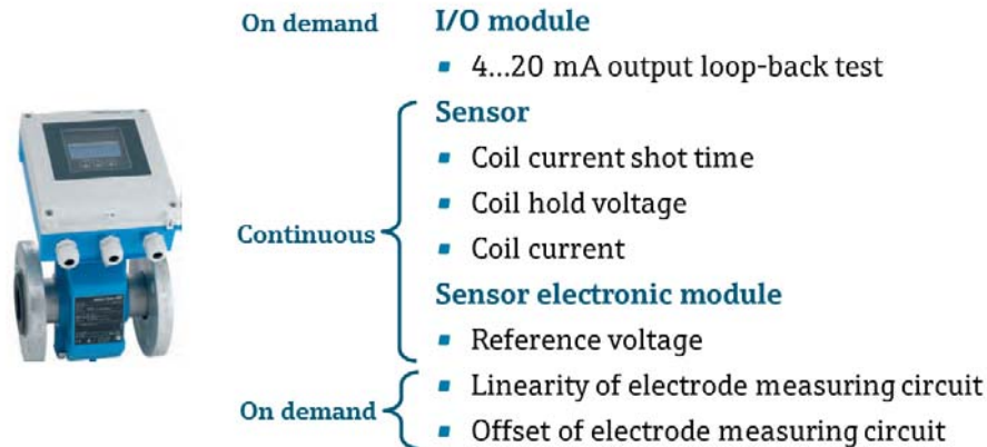
Proline Promag 400 example
